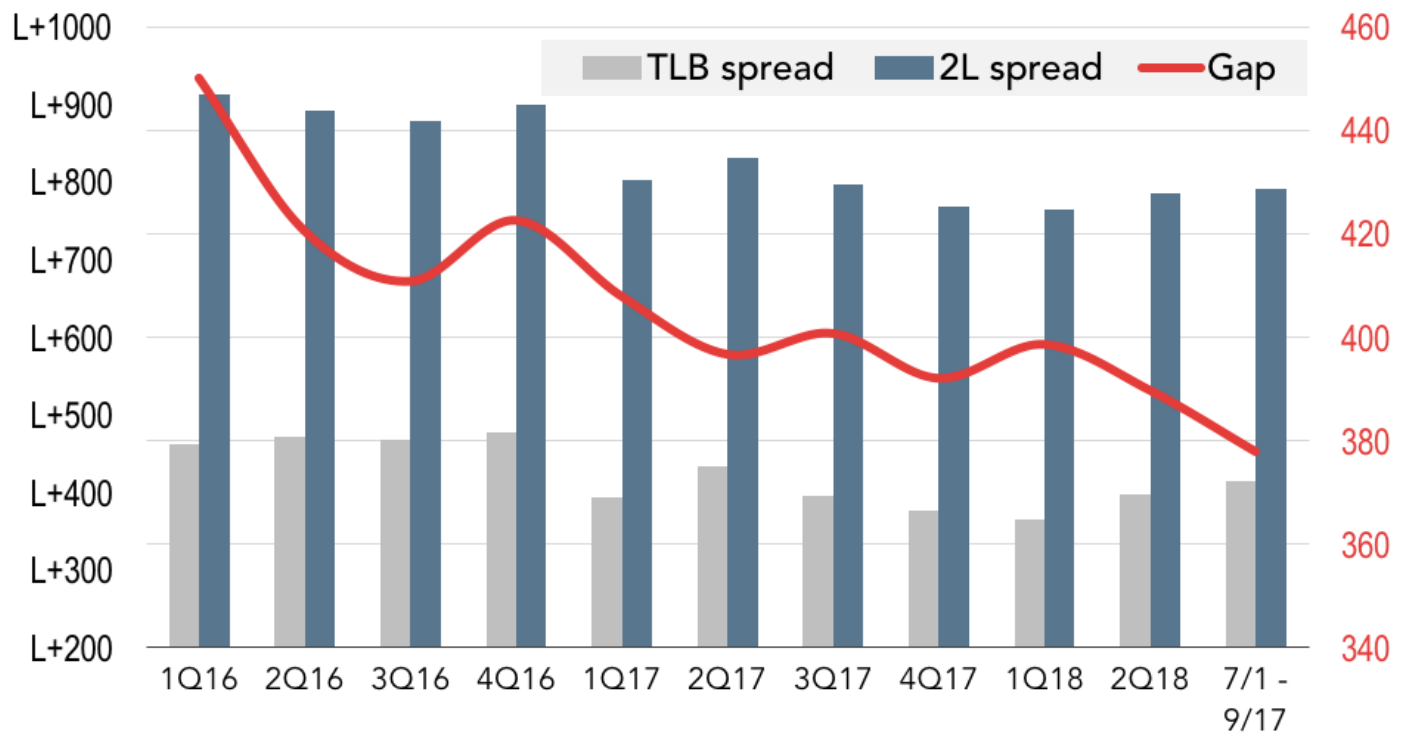
Spread of concurrent TLB & 2nd-lien loans
